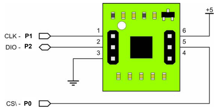
Figure 1. H48C Connections
